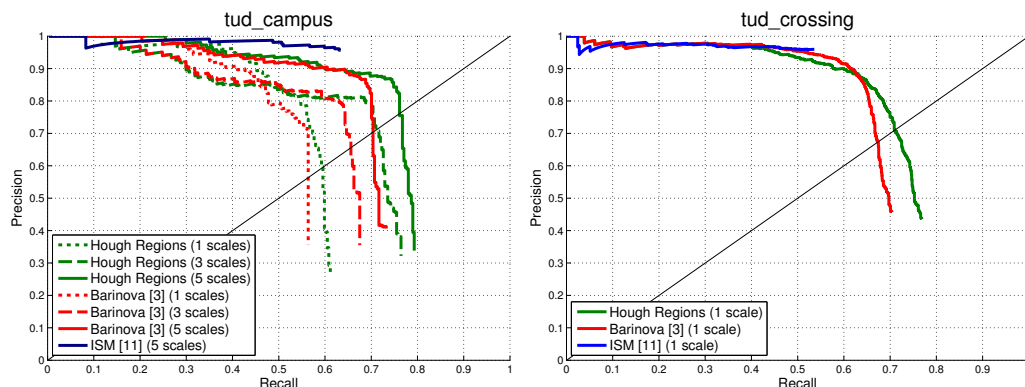
Figure 7.3: Object detection performance as Recall/Precision curve for the TUD campus and TUD crossing sequences showing analysis at multiple scales for highly overlapping instances. See text for details.
