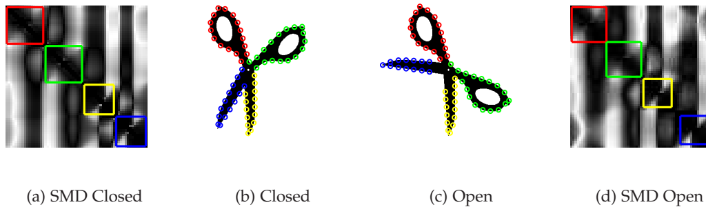
Figure 3.4: Articulation invariance is handled by returning a set of partially matching boundary parts. Corresponding boundary parts are depicted by the same color.
