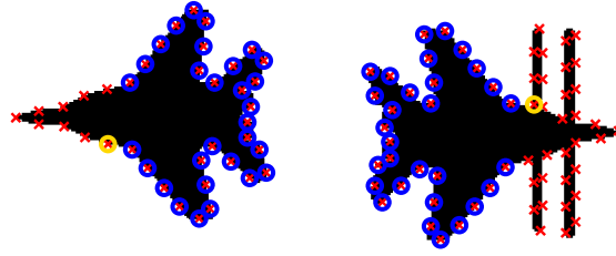
Figure 4.1: Result of our partial shape matching where sampled points are indicated by the crosses, and matching results are shown with circles.
