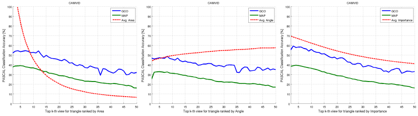
Fig. 5. Removing View Redundancy: showing accuracy for the single k -th ranked feature on x -axis (e.g. 1st largest area, 10th smallest angle, 4th learned importance) and average feature value (red dash). The smaller the area or the larger the angle, the worse performance gets. Our learned performance captures the combination of area and angle better. This is CamVid, other datasets are in supplemental material.
