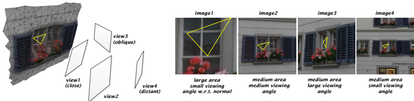
Fig. 4. Geometric link between 3D model and 2D image space. Contrary to related work in view clustering, we look for the best view c^*(f_i) per mesh triangle f_i . For small viewing angles the texture is visually pleasing but not best for semantic classification.
